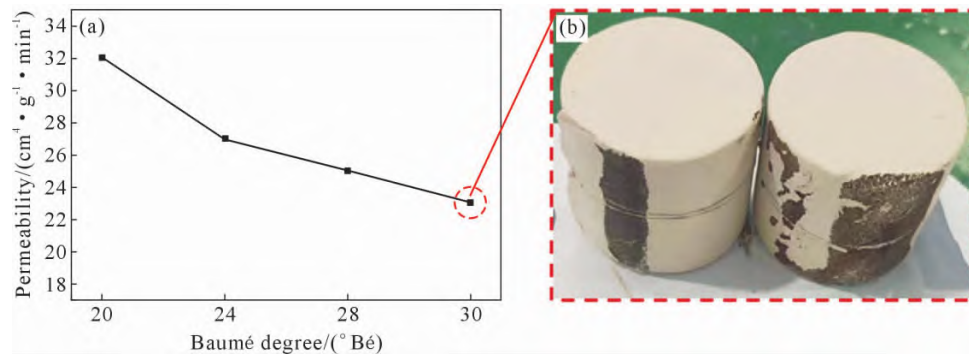
图6 不同波美度条件下砂型的透气性结果及高波美度条件下涂料涂挂烘干后的实物图:(a) 砂型透气性;(b) 实物图 Fig.6 Permeability results of the sand molds with different Baumé degrees and photographs of the coatings applied and dried with high Baumé degrees: (a) permeability results of the sand molds; (b) photograph
