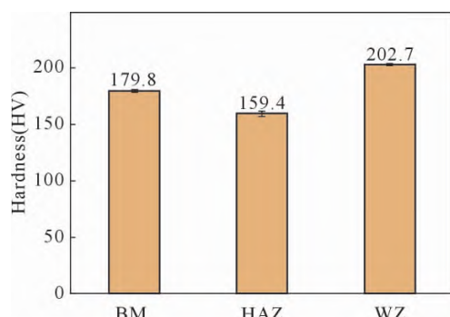
图 7 TIG 焊接 Zr-3 接头区域的硬度分布 Fig.7 Hardness distribution map of the TIG-welded Zr-3 joint zone
