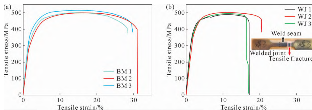
图5 TIG 焊接 Zr-3 母材与接头的拉伸应力-应变曲线:(a) 母材;(b) 焊缝 Fig.5 Tensile stress-strain curves of the Zr-3 base metals and weld joints by TIG: (a) base metal; (b) weld zone
