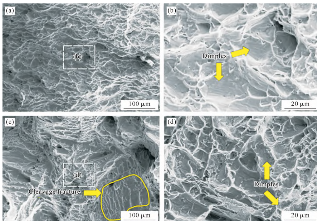
图 6 试样断口形貌 SEM 像:(a, b) 母材;(c, d) 焊缝 Fig.6 SEM images of the fracture morphology of the samples: (a, b) base metal; (c, d) weld zone
