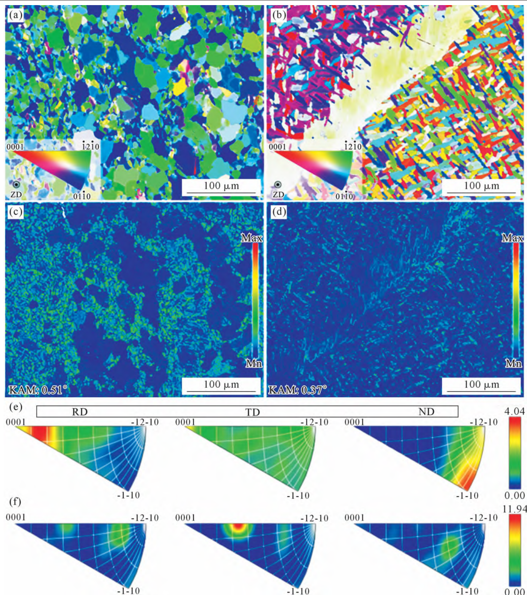
图3 母材与焊缝的IPF、KAM及PF图:(a, c, e)母材;(b, d, f)焊缝 Fig.3 IPF, KAM and PF maps of the base metal and weld zone: (a, c, e) base metal; (b, d, f) weld zone
