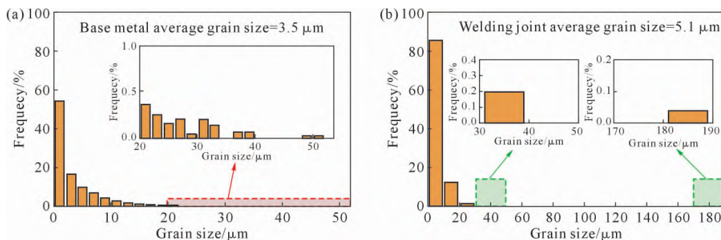
图4 母材与焊缝的晶粒大小尺寸分布:(a)母材;(b)焊缝 Fig.4 Size distribution of grains in the base metal and the weld zone: (a) base metal; (b) weld zone
