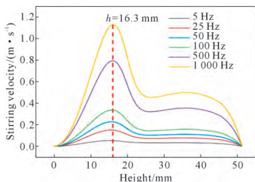
图11 不同频率下流场速度沿坩埚轴线分布曲线 Fig.11 Axial velocity distribution profiles along the crucible centerline under varying frequencies
