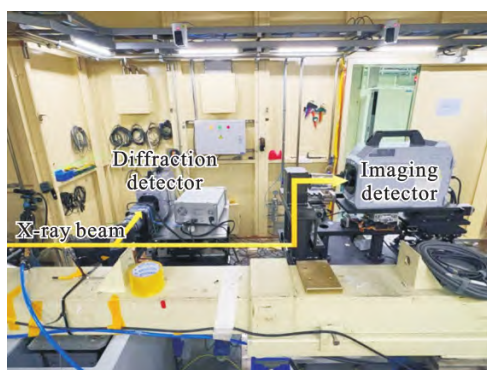
图 8 同步辐射衍射与成像协同 X 射线光路示意图 Fig.8 Schematic diagram of the X-ray optical path for synchronous radiation diffraction and imaging collaboration
