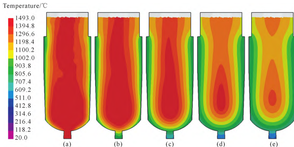
图 6 8 t 钢锭凝固过程的温度分布:(a) 充型结束,720 s;(b) 3 600 s;(c) 7 200 s;(d) 10 800 s;(e) 13 000 s Fig.6 Temperature distribution during solidification of the 8-ton steel ingot: (a) end of filling, 720 s; (b) 3 600 s; (c) 7 200 s; (d) 10 800 s; (e) 13 000 s
