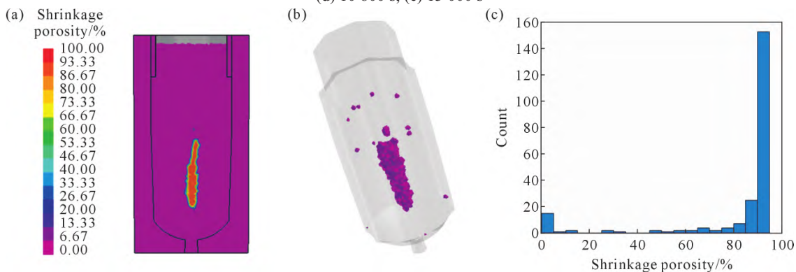
图 7 缩孔疏松分布:(a) 中心截面缩孔疏松分布;(b) 缩孔疏松三维分布;(c) 缩孔率大于零的分布 Fig.7 Shrinkage porosity distribution: (a) distribution on the central longitudinal section; (b) 3D distribution; (c) distribution of nodes with nonzero shrinkage porosity
