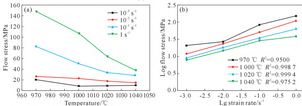
图6 变形温度和应变速率对 Ti150 合金流变应力的影响:(a) 变形温度;(b) 应变速率 Fig.6 Effects of deformation temperature and strain rate on the flow stress of the Ti150 alloy: (a) deformation temperature; (b) strain rate
