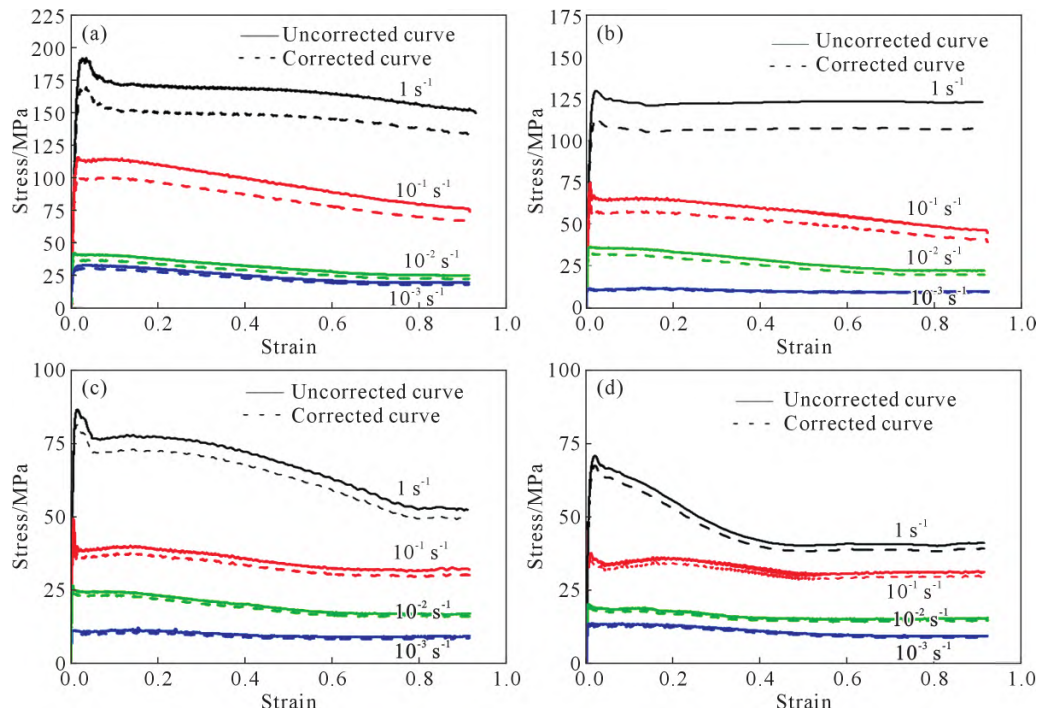
图5 Ti150 钛合金摩擦修正前后的应力-应变曲线:(a) 970 °C; (b) 1000 °C; (c) 1020 °C; (d) 1040 °C Fig.5 Stress-strain curves of the Ti150 titanium alloy before and after friction correction: (a) 970 °C; (b) 1000 °C; (c) 1020 °C; (d) 1040 °C
