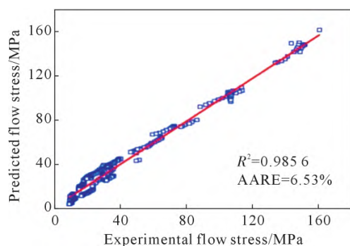
图 9 Ti150 钛合金预测和实验流变应力之间的相关性 Fig.9 Correlations between the predicted and experimental flow stresses for the Ti150 titanium alloy
