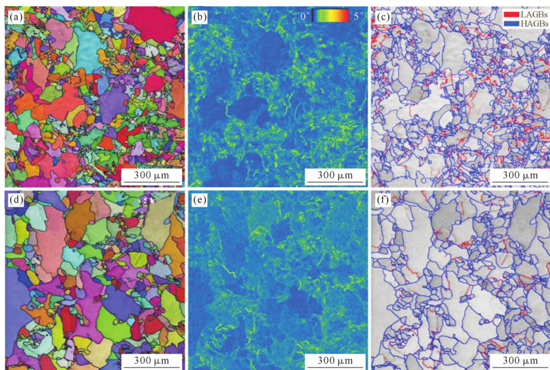
图6 激光定向能量沉积 Ti-6Al 合金样品 XOY 、 YOZ 面的 EBSD 分析: (a, d) IPF 图; (b, e) KAM 图; (c, f) 晶界取向图 Fig.6 EBSD analysis of the XOY and YOZ planes of the LDED Ti-6Al alloy: (a, d) inverse pole figure (IPF) images; (b, e) kernel average misorientation (KAM) maps; (c, f) grain boundary misorientation distributions
