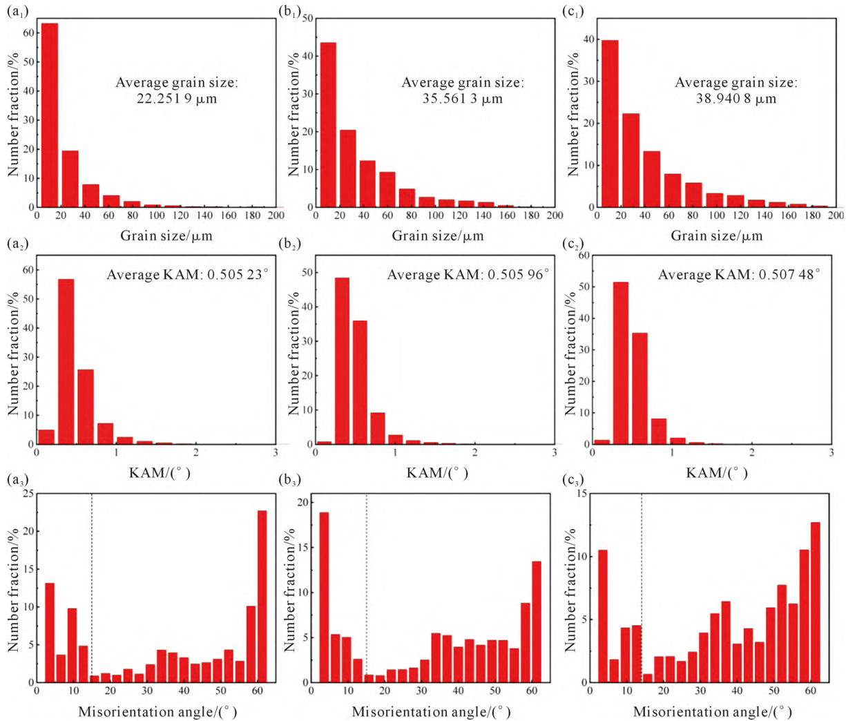
图7 激光定向能量沉积 Ti-6Al 合金样品晶粒尺寸、平均 KAM 及晶界取向分布: (a 1 ~a 3 ) XOY 面; (b 1 ~b 3 ) XOZ 面; (c 1 ~c 3 ) YOZ 面 Fig.7 The grain size, KAM and grain boundary misorientation distributions of the LDED Ti-6Al alloy: (a 1 ~a 3 ) XOY plane; (b 1 ~b 3 ) XOZ plane; (c 1 ~c 3 ) YOZ plane
