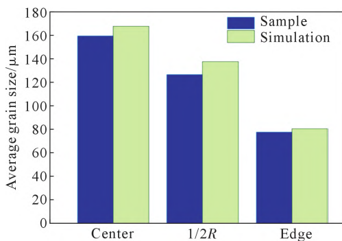
图6 实际与模拟晶粒尺寸对照图 Fig.6 Comparison between the actual and simulated grain
