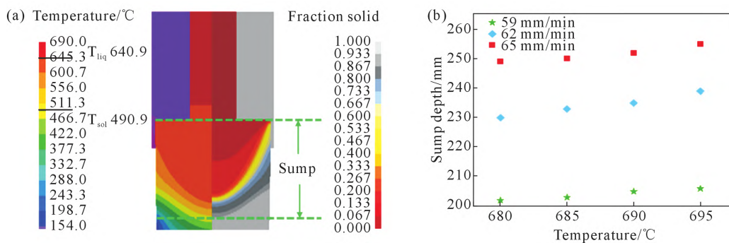
图10 不同工况下的液穴深度:(a)温度场与凝固场分布以及液穴深度,(b)不同工况的液穴深度 Fig.10 Sump under different working conditions: (a) temperature field and solidification field distribution and sump depth, (b) sump depth under different working conditions
