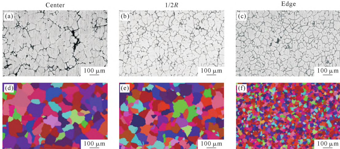
图5 实际与模拟晶粒形貌对照图:(a~c)中心、1/2R及边缘处金相图,(d~f)中心、1/2R及边缘处凝固组织模拟图 Fig.5 Comparison of actual and simulated grain morphology: (a~c) OM image at the center, 1/2R and edge, respectively, (d~f) simulation diagram of the solidification structure at the center, 1/2R and edge, respectively
