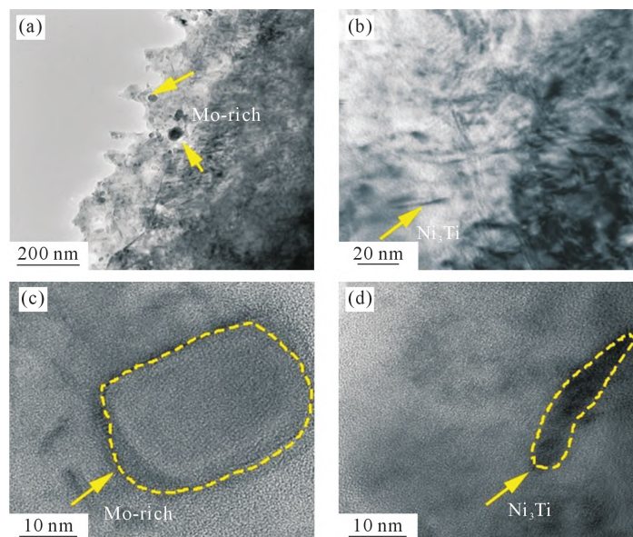
图5 Co-1试样的析出相TEM表征结果:(a)富Mo相低倍形貌,(b)Ni 3 Ti相低倍形貌,(c)富Mo相高分辨图,(d)Ni 3 Ti相高分辨图
