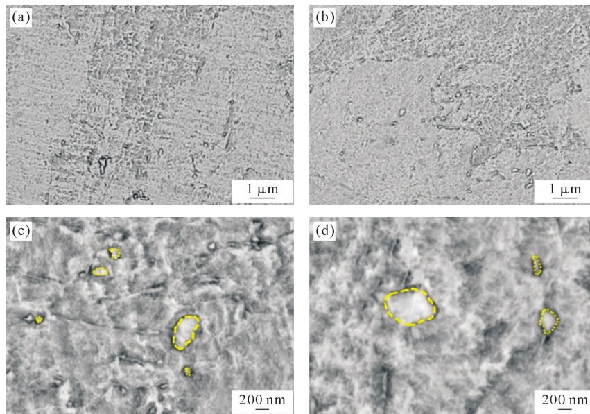
图4 析出相的SEM表征结果:(a) Co-1试样-低倍,(b) Co-5试样-低倍,(c) Co-1试样-高倍,(d) Co-5试样-高倍 Fig.4 SEM images of precipitated phases: (a) Co-1 specimen-low magnification, (b) Co-5 specimen-low magnification, (c) Co-1 specimen-high magnification, (d) Co-5 specimen-high magnification
