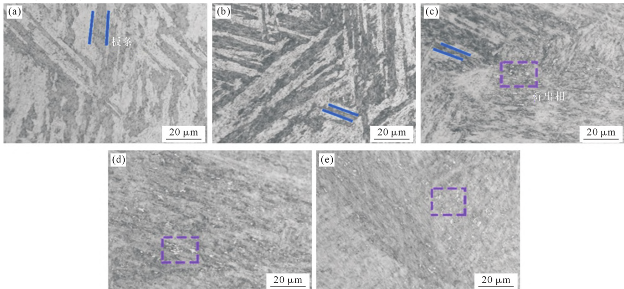
图2 时效组织高倍光镜形貌:(a) Co-1, (b) Co-2, (c) Co-3, (d) Co-4, (e) Co-5
