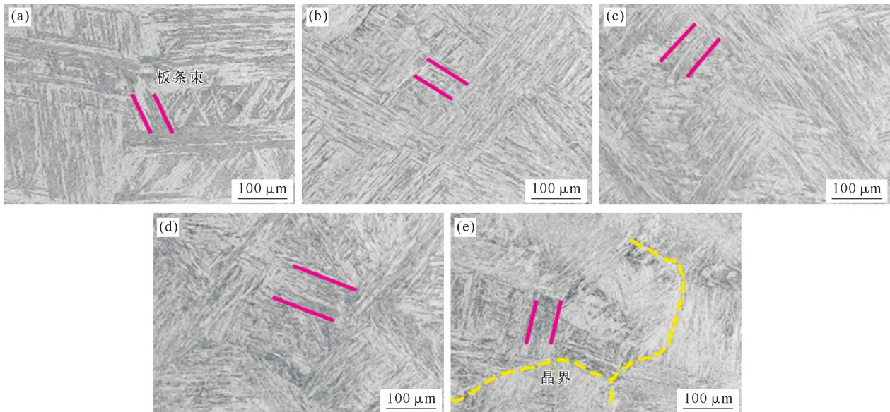
图1 时效组织低倍光镜形貌:(a) Co-1, (b) Co-2, (c) Co-3, (d) Co-4, (e) Co-5
