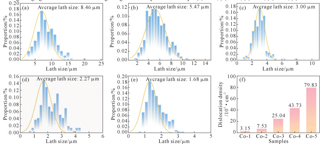
图3 不同Co含量下马氏体时效钢的板条宽度以及位错密度柱状图:(a) Co-1, (b) Co-2, (c) Co-3, (d) Co-4, (e) Co-5, (f) 位错密度 Fig.3 Histograms of lath width and dislocation density of the maraging steels with different Co contents: (a) Co-1, (b) Co-2, (c) Co-3, (d) Co-4, (e) Co-5, (f) dislocation density
