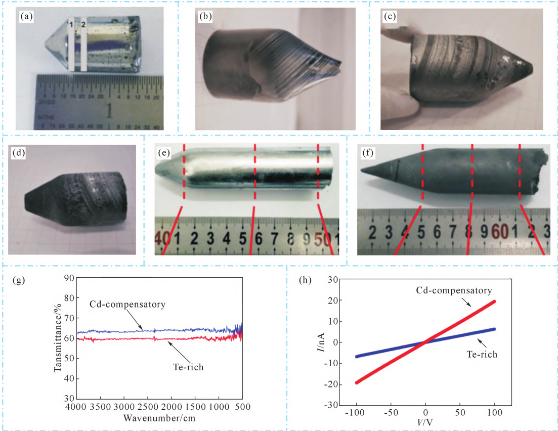
图5 CdMgTe晶体及其性能:(a)直径为18mm的In掺杂CdMgTe晶锭,(b~d) \text{Cd}_{1-x}\text{Mg}_x\text{Te} 晶体在蚀刻后显示孪晶和晶界( x=0.04, 0.08, 0.10 ),(e~f)两个 \text{Cd}_{1-x}\text{Mg}_x\text{Te} 晶锭在不同条件下生长的照片(Cd过量和富Te条件),(g) \text{Cd}_{1-x}\text{Mg}_x\text{Te} 晶体的IR透射率曲线,(h) \text{Cd}_{1-x}\text{Mg}_x\text{Te} 晶体的典型 I - V 曲线 [58-60] Fig.5 CdMgTe crystals and their performances: (a) 18 mm diameter In-doped CdMgTe ingot, (b~d) \text{Cd}_{1-x}\text{Mg}_x\text{Te} crystals after etching revealing twins and grain boundaries ( x=0.04, 0.08, 0.10 ), (e~f) pictures of the two \text{Cd}_{1-x}\text{Mg}_x\text{Te} ingots grown under different conditions (Cd excess and Te-rich conditions), (g) IR transmittance curves of the \text{Cd}_{1-x}\text{Mg}_x\text{Te} crystals, (h) typical I - V curves of the \text{Cd}_{1-x}\text{Mg}_x\text{Te} crystals [58-60]
