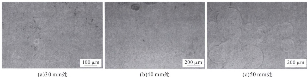
图 5 (\text{Cu}_{43}\text{Zr}_{48}\text{Al}_9)_{98}\text{Y}_2 不同位置的金相图 Fig.5 Microstructure in different position of (\text{Cu}_{43}\text{Zr}_{48}\text{Al}_9)_{98}\text{Y}_2
