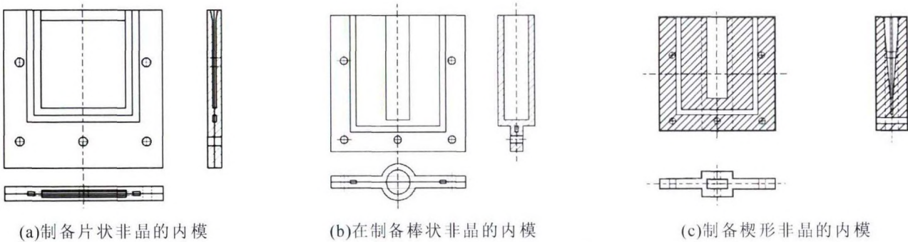
图 2 具有不同型腔的内模 Fig.2 Internal mold with different cavities
