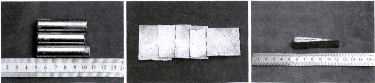
图 3 采用新设计模具制备的不同形状块体非晶材料 Fig.3 Different shapes of bulk amorphous materials prepared by using new design molds
