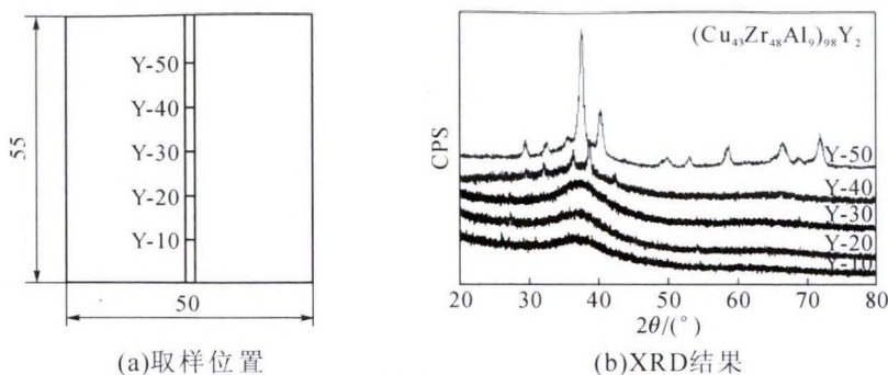
图 4 板状非晶 XRD 检测取样示意图和 XRD 分析结果 Fig.4 Schematic diagram of plate-like amorphous XRD test samples and XRD analysis results
