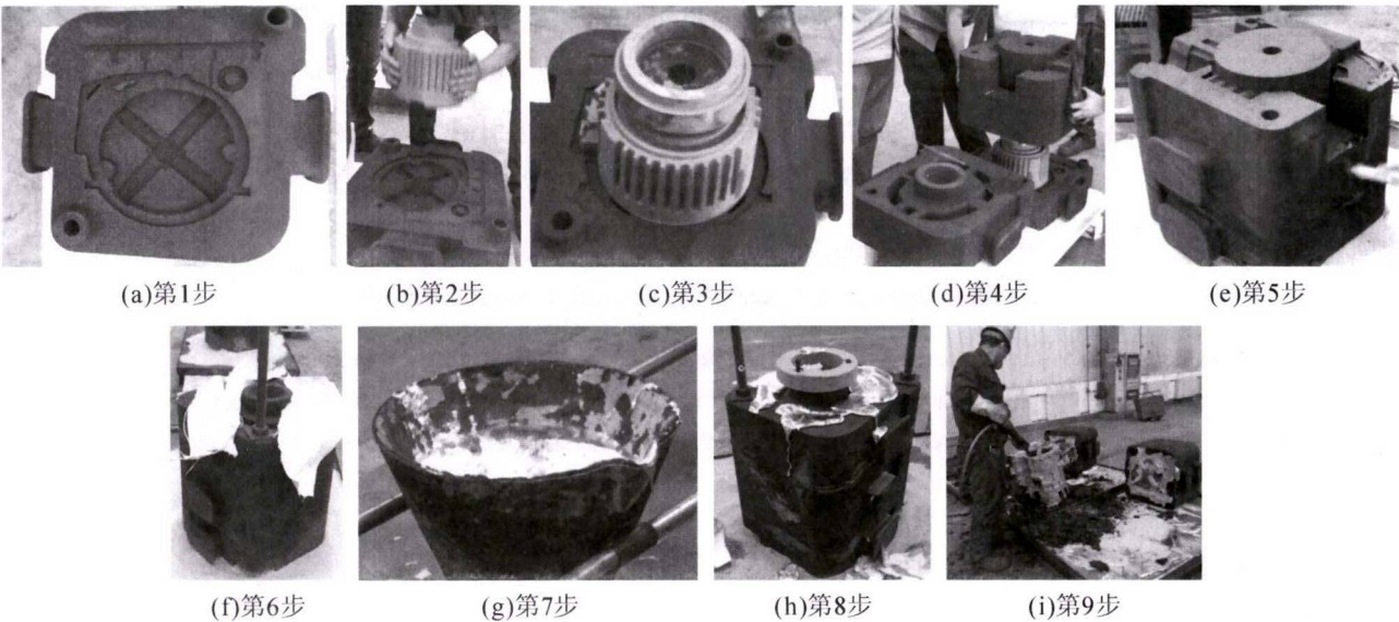
图 8 组芯浇注工艺步骤 Fig.8 Core assembly and pouring processes
