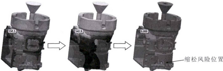
图 5 铸件壳体凝固过程模拟结果 Fig.5 Simulated result of solidification of casting
